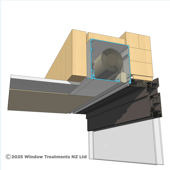
Modular Single Recess Flush Box
