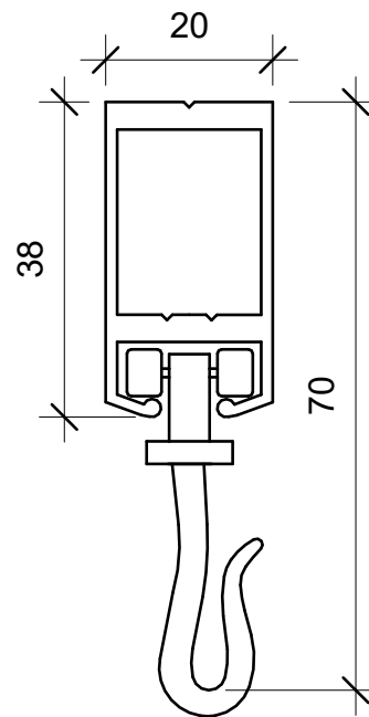
Movatrack Profile Roller Wheel and Curtain Hook Scale 1:1
