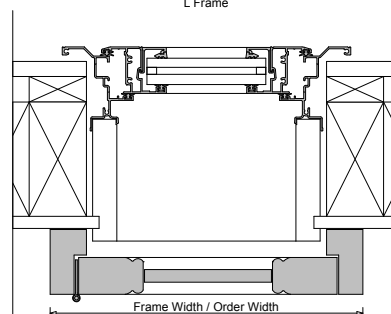
Outside Mount L Frame
