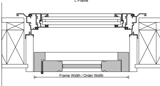
Inside Mount L Frame
