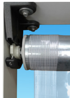
Heavy Duty Mounting Bracket, Reinforcing strip
